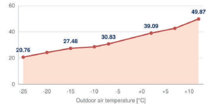
Heating capacity [kW] — EN 14511-2
